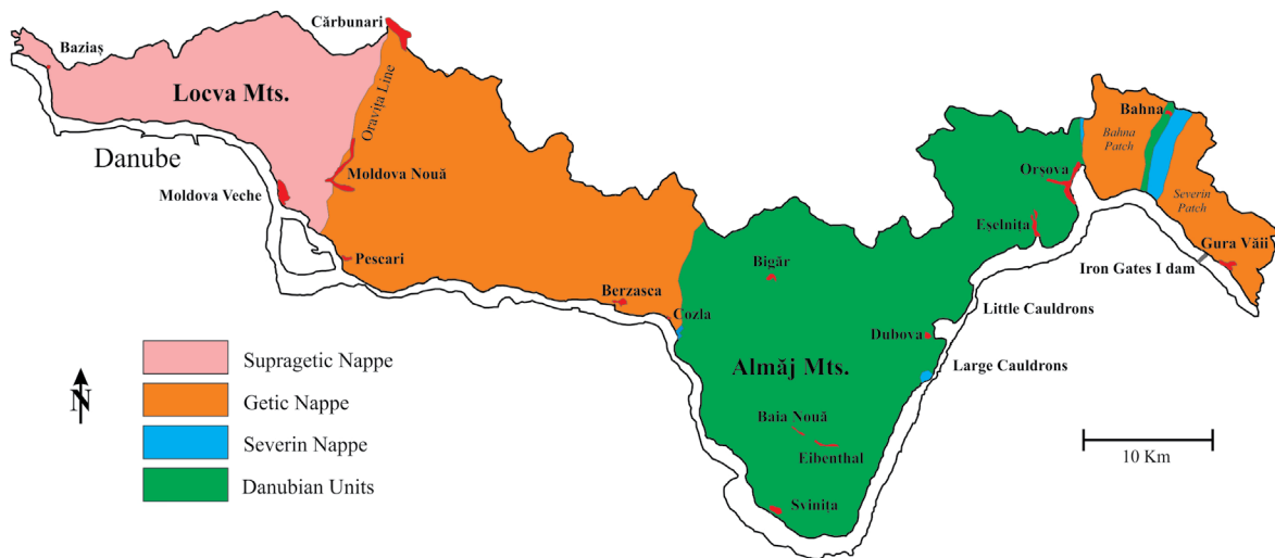
Fig. 13 Tectonic sketch of Iron Gates Natural Park. Tectonic units (Supragetic, Getic, Severin Nappes, and the Danubian Units) are illustrated without their post-tectonic (Mio-Pliocene) sedimentary fillings. The colors are correlated with those in Fig. 14, and 15
