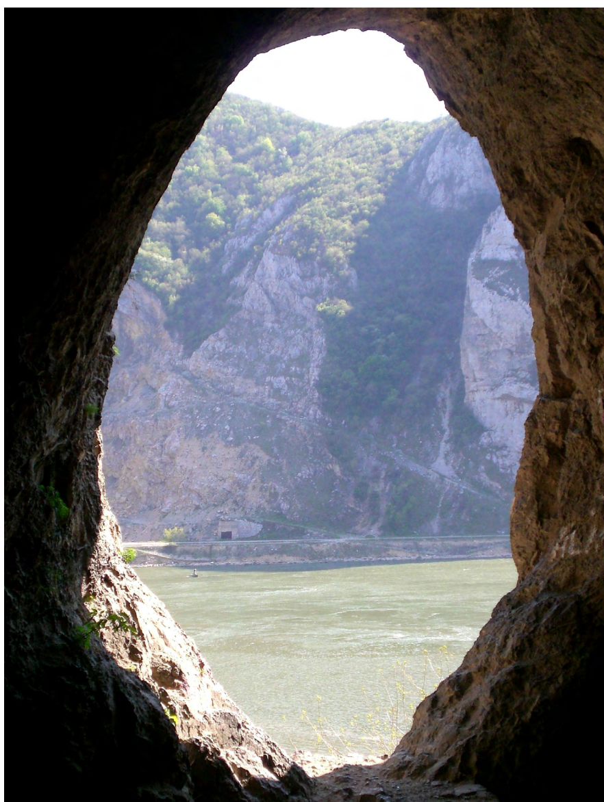
Fig. 20 Gaura cu Muscă cave in Cretaceous limestone of the Reșița Basin, Getic Nappe
