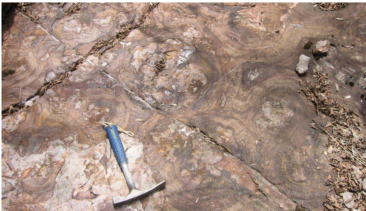
Fig. 47 Middle Jurassic stromatolites (organic-sedimentary structures), Saraorschi SSSI, close to Svinița, Sirinia Basin, Danubian Units
