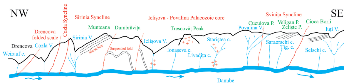
Fig. 17 Simplified morphological sketch of the Danube valley, with significant tectonic bodies, modified after Codarcea et al. (1961) and Mutihac (1990)
